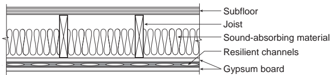
Figure 3. Resilient metal channels between two layers of 15.9-mm fire-rated gypsum board in the ceiling give this construction an STC of only 38. As shown in Table 4, removing the internal layer of gypsum board gives an STC of 52 for an OSB subfloor. Putting both layers below the resilient metal channels gives an STC of 55.
