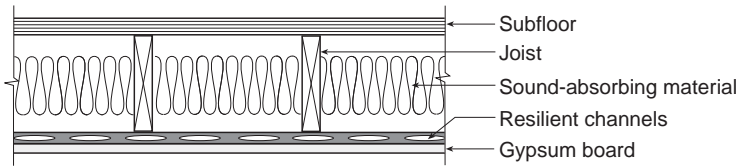
Figure 1. A generic joist floor. Resilient metal channels support one or more layers of gypsum board below the joist, which can be of any type. The sound-absorbing material in the cavity increases the sound isolation when resilient channels are present.
