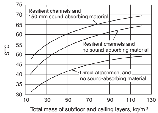
Figure 2. Dependence of STC on total mass per square metre of subfloor and ceiling layers for uniformly spaced resilient metal channels (610 mm o.c.)
